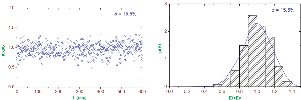
Fig. 9. Pulse-to-pulse fluctuation of SASE pulse energy in saturation regime. The electron beam was in short bunch setting, cf. the upper plots in Figure 8. The solid line represents a numerical simulation with the code FAST [32].
