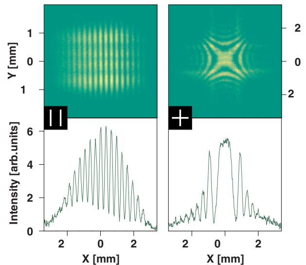
Fig. 10. Diffraction patterns of two different slit arrangements (see pictographs) illustrating the transverse coherence of the FEL radiation; left: double slit, each slit 2 mm (vert) \times 200 \mu\text{m} (horiz.), horizontal slit separation 1 mm; right: crossed slits, each slit 4 mm \times 100 \mu\text{m} . The slits are located 12 m behind the exit of the undulator. The images have been recorded with a gated CCD camera viewing a Ce:YAG fluorescent screen 3 m behind the slits. They have been taken as a sum of a few consecutive FEL pulses with a wavelength of 95 nm. The lower part of both images depicts a horizontal cut through the centre of the respective diffraction pattern.
