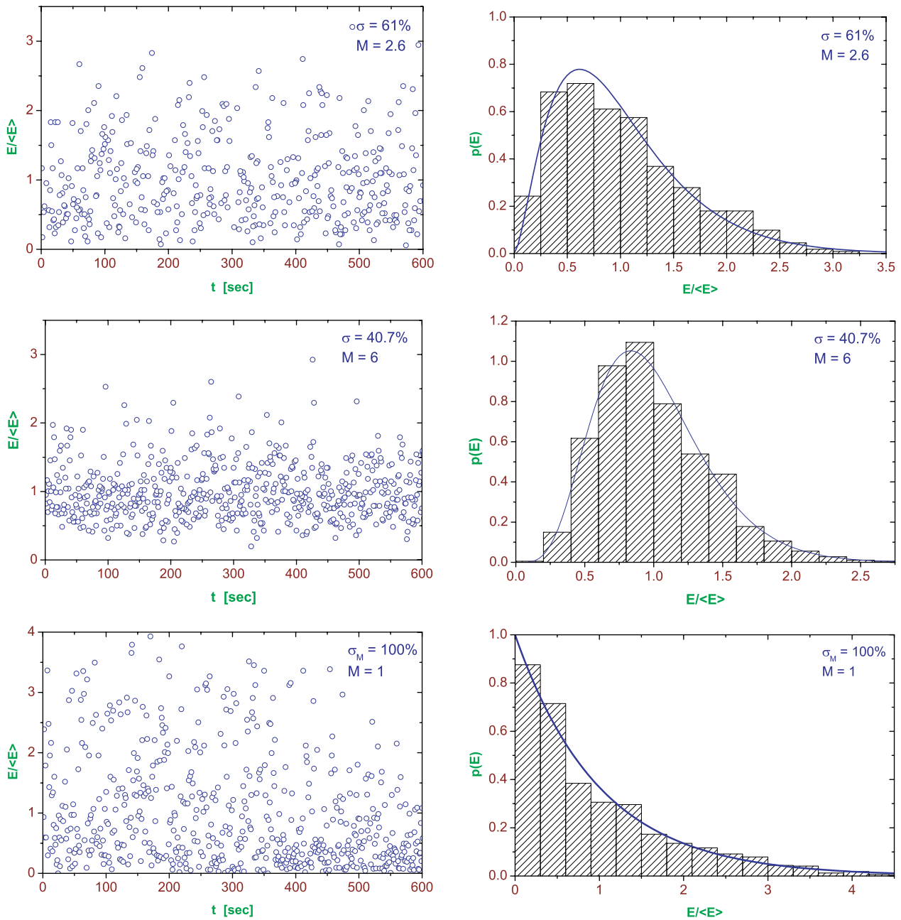
Fig. 8. Pulse-to-pulse fluctuation of SASE pulse energy for different settings of electron bunch length. Left column: measured single pulse energy versus time; right column: histogram of probability distribution extracted from the measurement. The SASE pulses are observed at high gain, but still in the exponential regime, not yet in laser saturation, cf. Figure 5. The upper plot is for short electron bunch setting (equal to the setting used for Fig. 7, top), the middle plot is for long electron bunch setting (equal to the setting used for Fig. 7, bottom), and the lower one is for the radiation pulse having passed a narrow-band monochromator. The solid curves represent gamma distributions according to equation (3) with the mode number M = \sigma^{-2} calculated from the standard deviation \sigma of each distribution.
