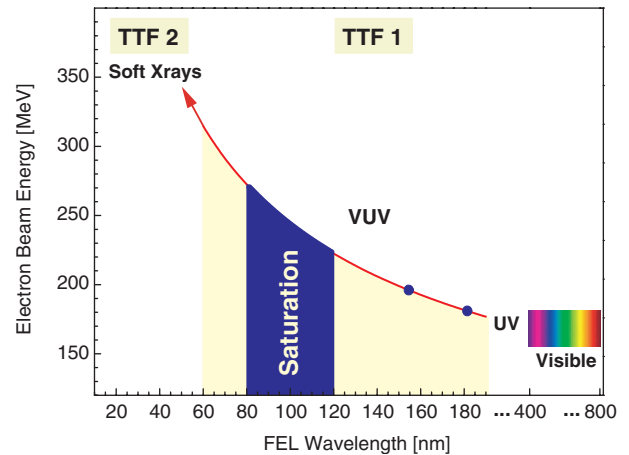
Fig. 4. VUV wavelength range within which lasing has been obtained at the TTF FEL, phase 1 (TTF1). The wavelength was tuned by changing the electron beam energy (vertical axis, cf. Eq. (1)). The individual dots outside the range in which saturation has been achieved represent an FEL gain of typically > 1000 demonstrated in an earlier stage of the experiment [30]. After a linac upgrade to electron beam energies of up to 1 GeV (TTF 2), the FEL will enter the soft X-ray region [18].
